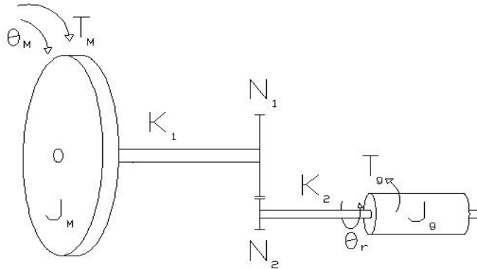
Fig. 2. Drive train model
