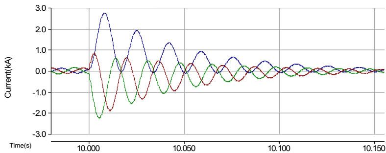
Fig. 11. Fault current contribution from an induction generator
