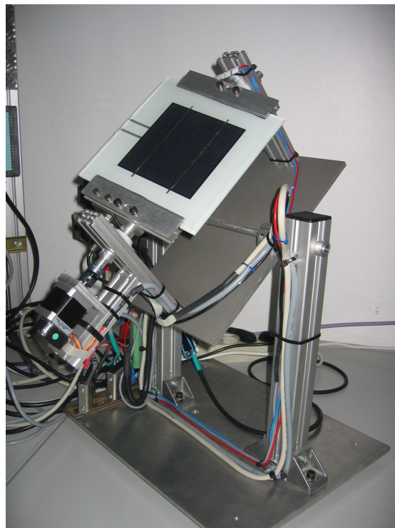
Fig. 6. Built Prototype: Global view
