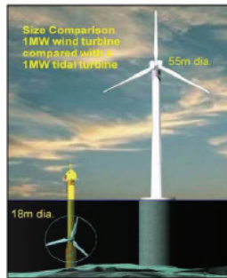
Fig. 8. Tidal turbine in comparison with offshore wind turbine
