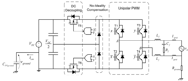
Fig. 18. Schematic of the original configuration for full bridge topology with unipolar PWM for transformerless converters.
