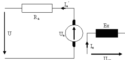
Fig. 6. Equivalent circuit diagram of a small wind generator
