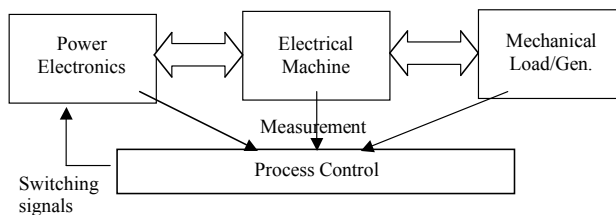
Fig. 2. The Electrical Drive structure.
