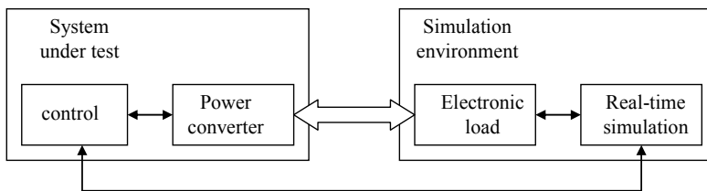
Fig. 5. Power Level HIL simulation.
