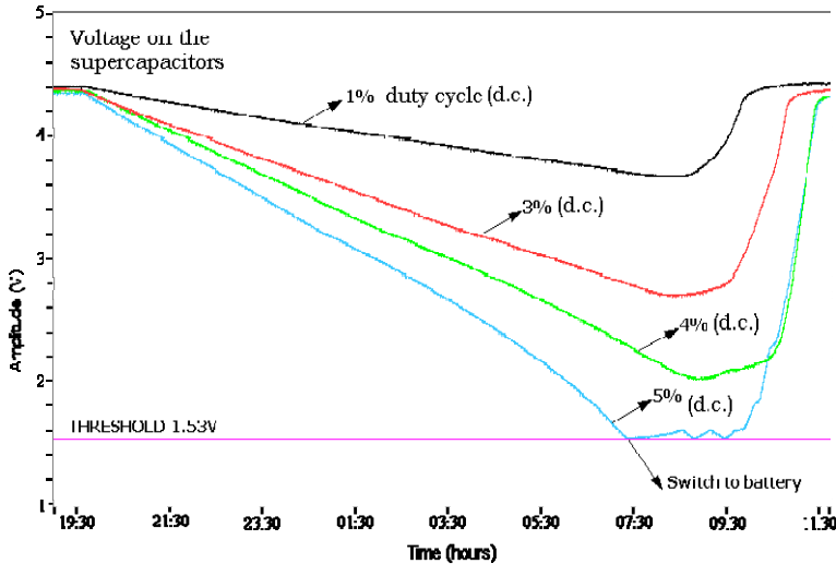
Fig. 7. This figure shows the discharge of the supercapacitors during 4 nights overlapped at different load currents. Each curve belongs to a different night.
