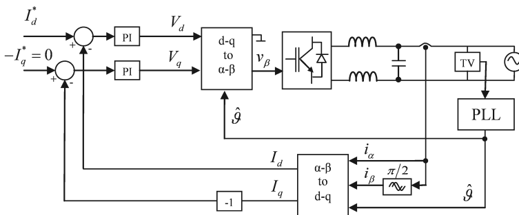
Fig. 5. Block diagram of d-q control structure.
