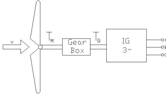
Fig. 1. Basic wind turbine system model
