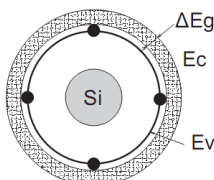
Fig. 2. Atom of silicon with represented energy levels.
