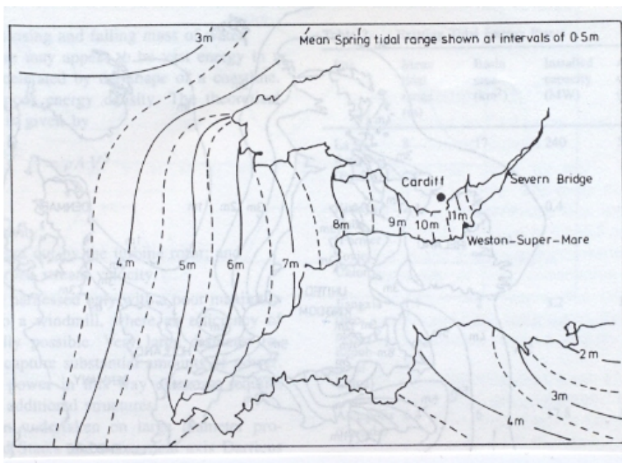
Fig. 13. Tidal Resonance in the Severn Estuary.
