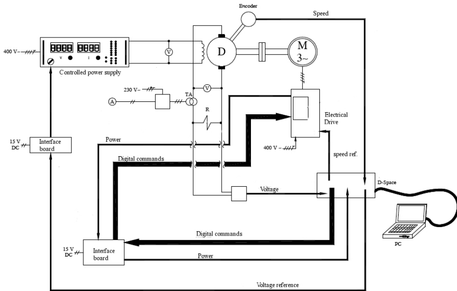
Fig. 18. Example of mechanical HIL test bench
