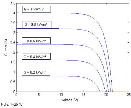
Fig. 4. PV module I-V characteristics for different illumination
