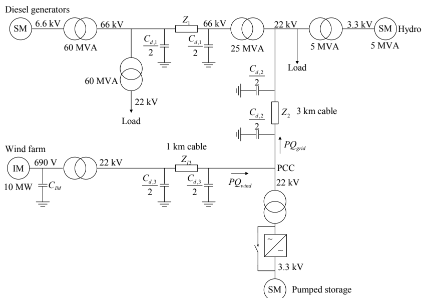
Fig. 7. Simplified grid model of the isolated system used for the presented simulations (Suul, 2006)
