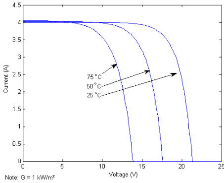
Fig. 3. PV module I-V characteristics for different temperature
