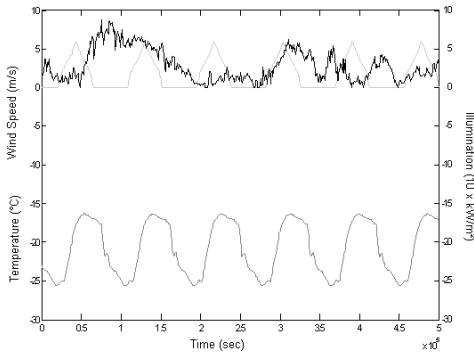
Fig. 10. Wind speed, temperature and illumination in January
