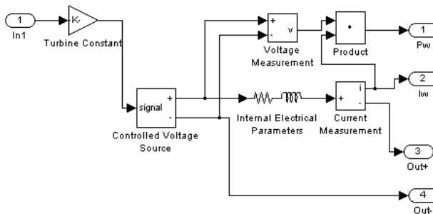
Fig. 7. Matlab-Simulink model of the generator
