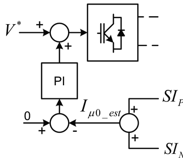
Fig. 14. Block diagram of the saturation compensation scheme.
