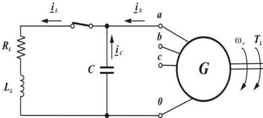
Fig. 3. Single-phase R-L load circuit
