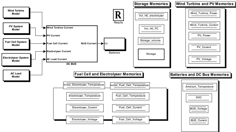
Fig. 9. Matlab/Simulink simulation model of the renewable energy system
