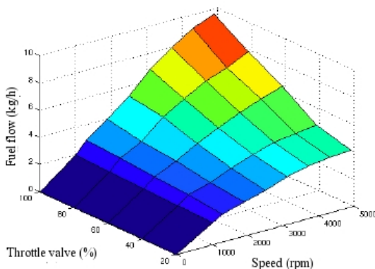
Fig. 20. Fuel flow vs. speed and throttle valve opening.
