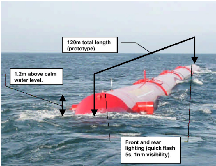
Fig. 5. OPD Pelamis WEC Device.
