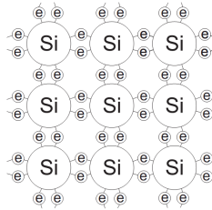
Fig. 3. Atoms of silicon inside intrinsic semiconductor.
