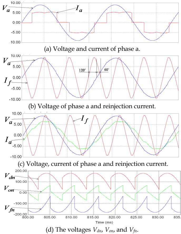
Fig. 3. Various voltages and currents of the proposed approach at \alpha=20^\circ .
