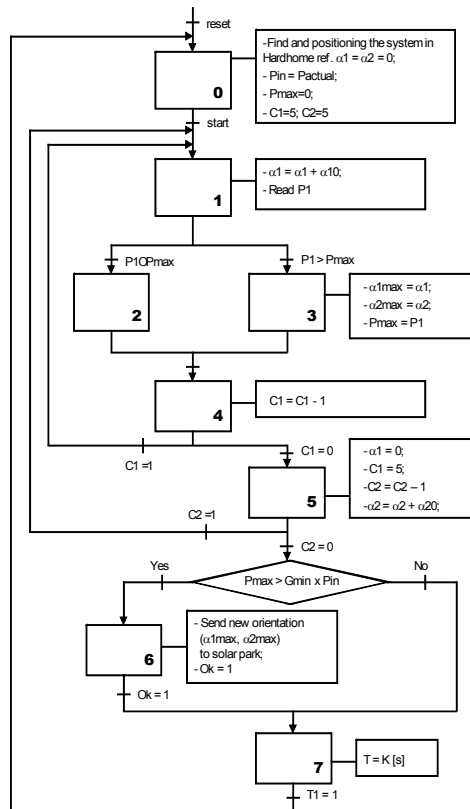
Fig. 7. Control Algorithm for the Tracking System
