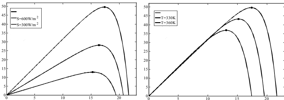
Fig. 15. SHELL Q8 PV V/I characteristics.
