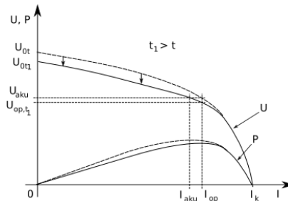
Fig. 25. Effect of temperature change on VoltAmper characteristics of a typical photovoltaic cell.
