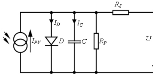
Fig. 1. Equivalent circuit diagram of a solar cell
