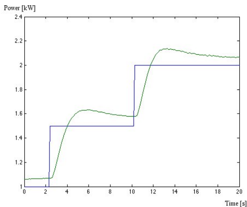
Fig. 22. Power reference and generated power vs. time.
