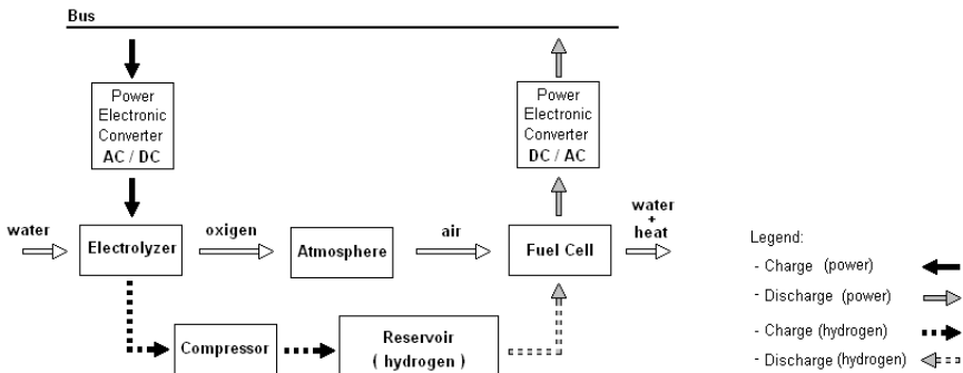
Fig. 11. Hydrogen fuel cell energy storage system operation diagram
