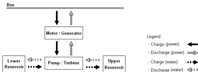
Fig. 8. Pumping hydro system operation diagram
