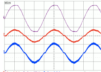
(b) PI regulator + feed forward control with saturation compensation
