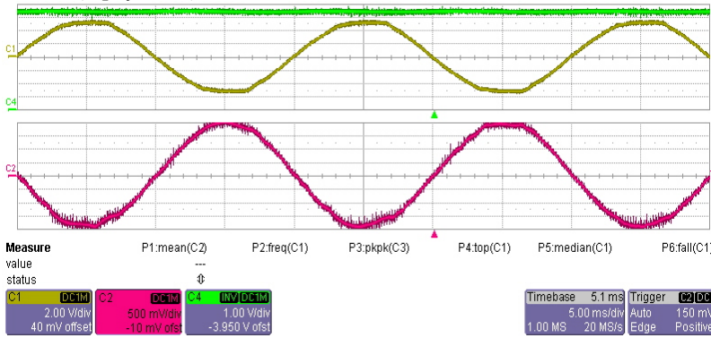
Fig. 18. Steady-state operation of RES in regime of active power delivering: voltage (top) and current (bellow)
