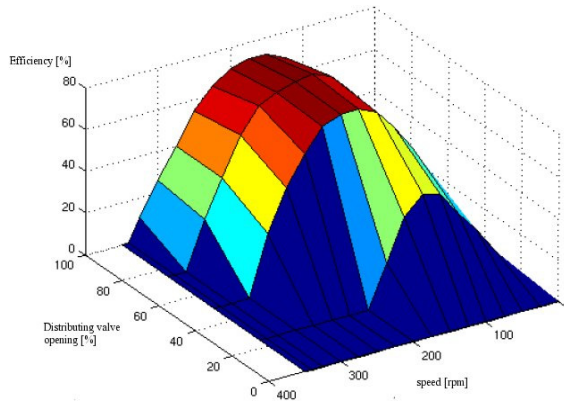
Fig. 21. Efficiency vs. turbine speed and distributing valve opening.
