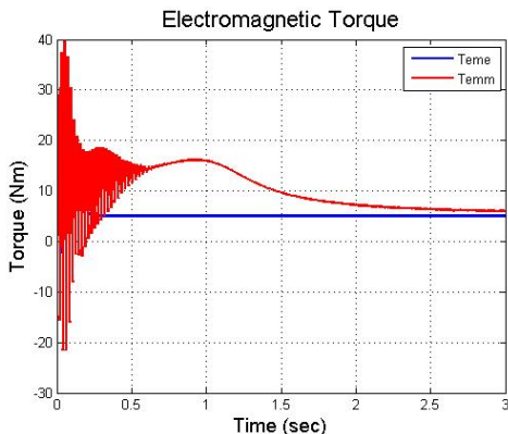
Fig. 11. Estimated electromagnetic torque using EKF
