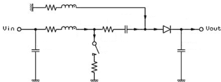
Fig. 6. SEPIC topology
