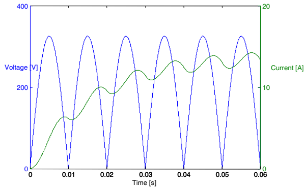
Fig. 6. Dynamic state of connecting nonlinear rectifying load to RES: voltage on DC side (blue) and DC current (green)
