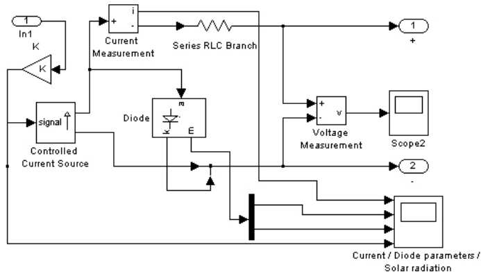
Fig. 3. Matlab Simulink implementation of the PV module.
