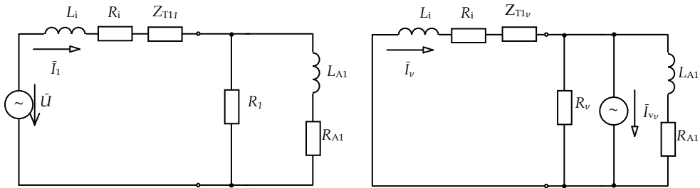
Fig. 4. a,b Equivalent scheme for fundamental (a) and \nu - harmonic (b) components of one appliance, where \tilde{U} is complex magnitude of network voltage source with voltage of fundamental current source representing nonlinearity of appliance, \tilde{I}_1 and \tilde{I}_\nu are complex magnitudes of network current for fundamental and \nu - harmonic component, \tilde{I}_{\nu\nu} is complex magnitude of current source representing nonlinearity of appliance
