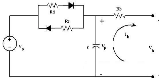
Fig. 9. Thevenin equivalent battery model.
