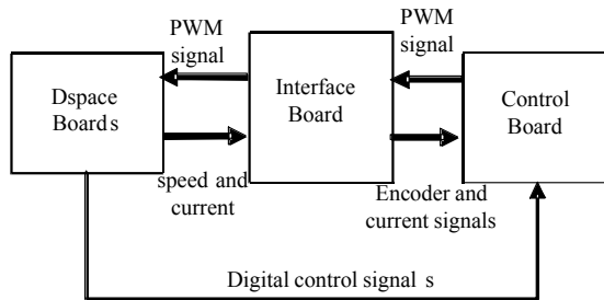
Fig. 11. Signal level HIL test bench architecture.
