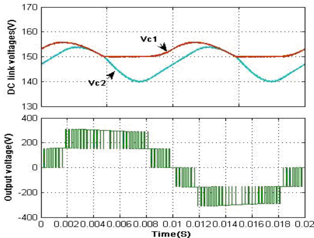
Fig. 23. Capacitor voltage balancing in three-level diode-clamped Inverter with double-output boost converter
