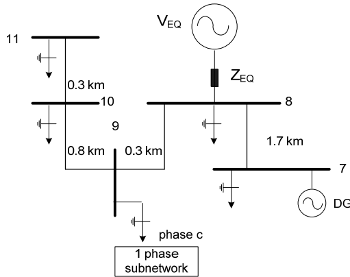
Fig. 5. Simplified distribution system
