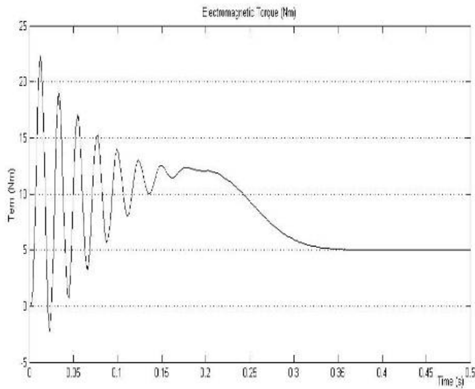
Fig. 20. Estimated electromagnetic torque using U_s\text{-}\omega estimator
