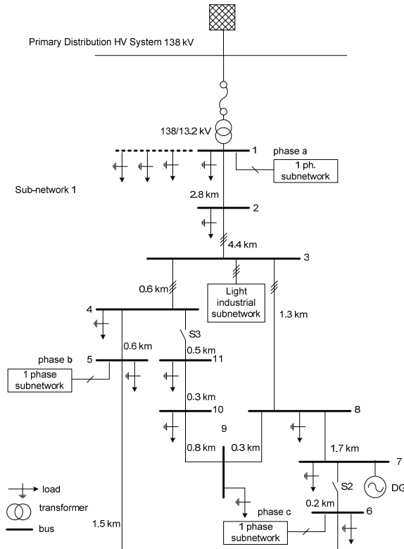
Fig. 4. Medium voltage distribution system
