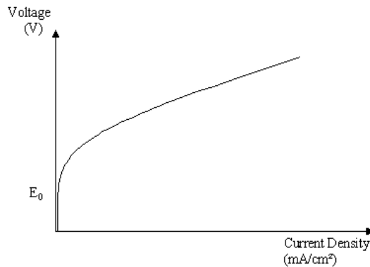
Fig. 6. Electrolyzer polarisation characteristic
