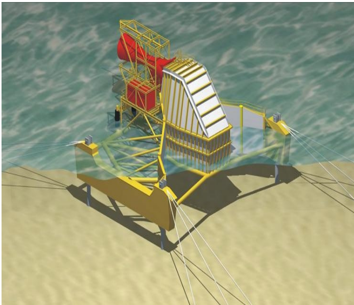
Fig. 6. Energetech WEC Device.
