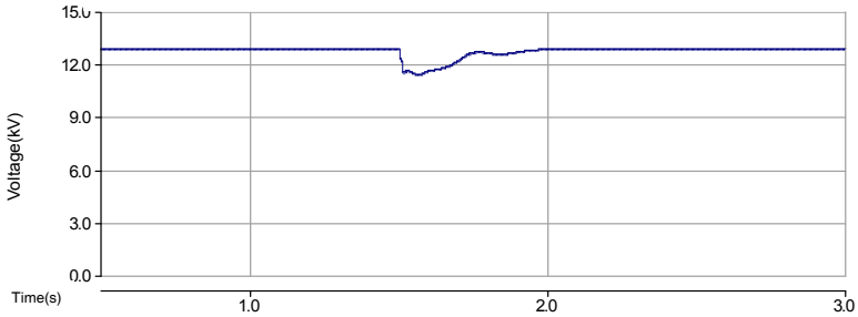
Fig. 6. Voltage at bus 11 during the wind generator start-up.
