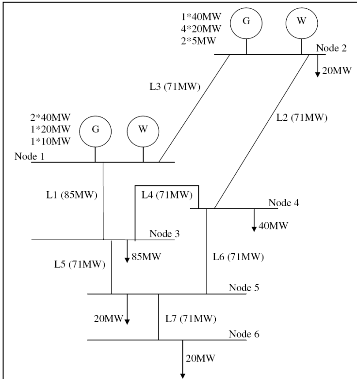
Fig. 10. Implemented version of the RBTS
