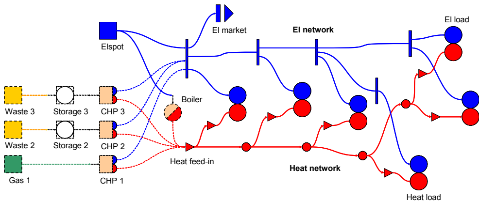
Fig. 3. Energy supply system layout
