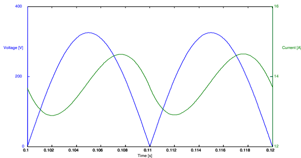
Fig. 7. Steady-state time-vaweforms of DC voltage (blue) and current (green)
