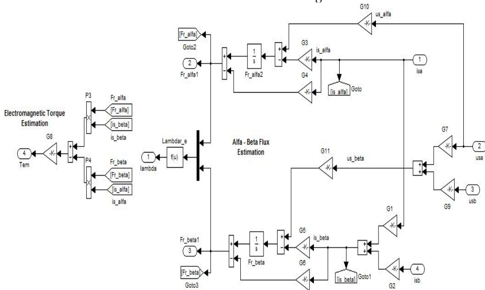
Fig. 13. U_s - I_s estimator Simulink model
