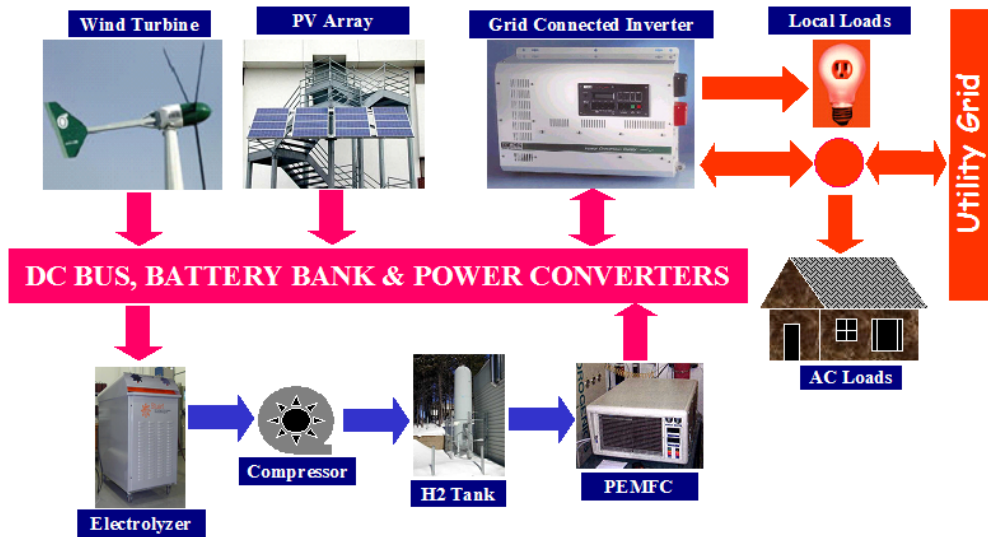
Fig. 22. Grid-connected renewable energy system with hydrogen storage
