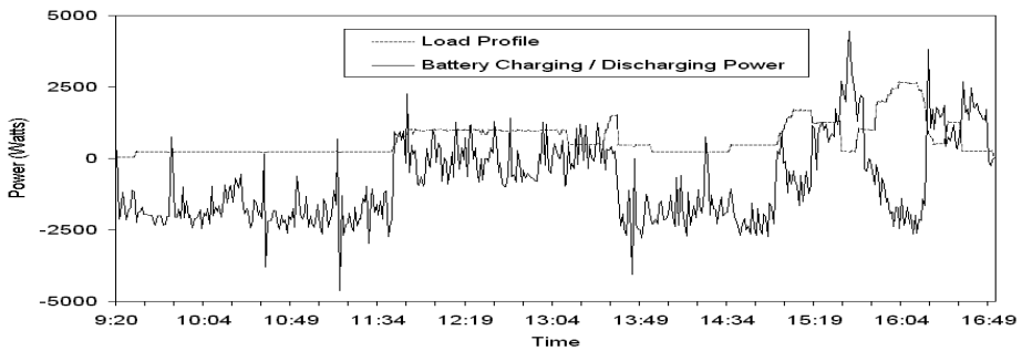
Fig. 21. Load and batteries powers
