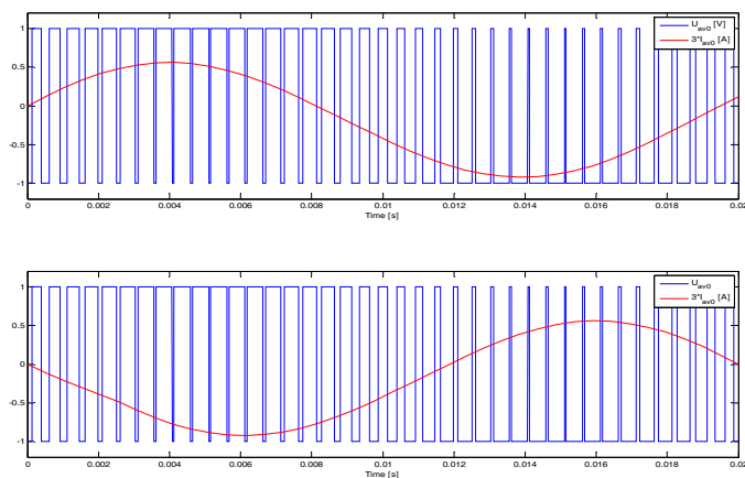
Fig. 9. Time-waveforms of output voltage (blue) and current (red) for generating and regenerating regimes (considering 999 harmonics)
