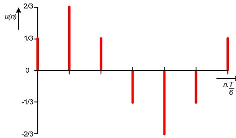
Fig. 10. Switching function for three-phase 6-pulse RES inverter
