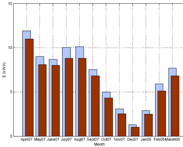
Fig. 34. Energy produced in individual months in a year.
