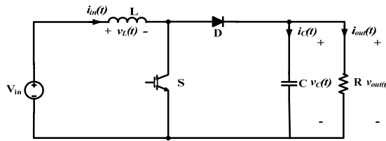
Fig. 4. Schematic configuration of a DC-DC boost converter
