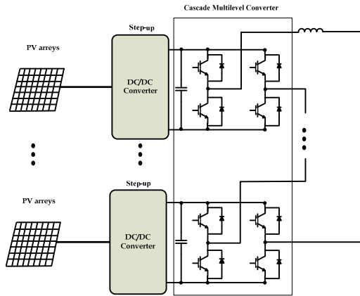
Fig. 16. Multilevel converter in transformerless PV systems
