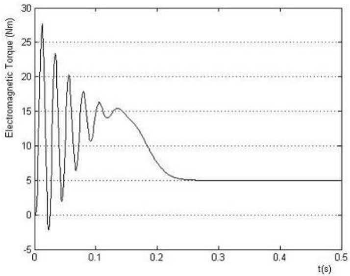
Fig. 16. Estimated electromagnetic torque using U_s - I_s estimator
