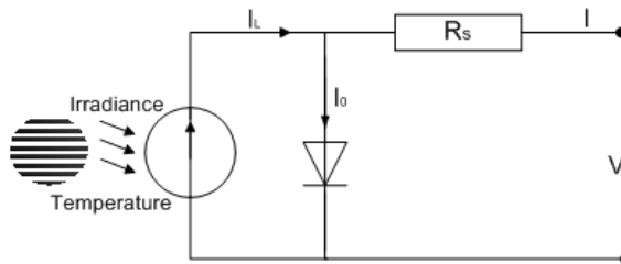
Fig. 2. Circuit diagram of PV model
