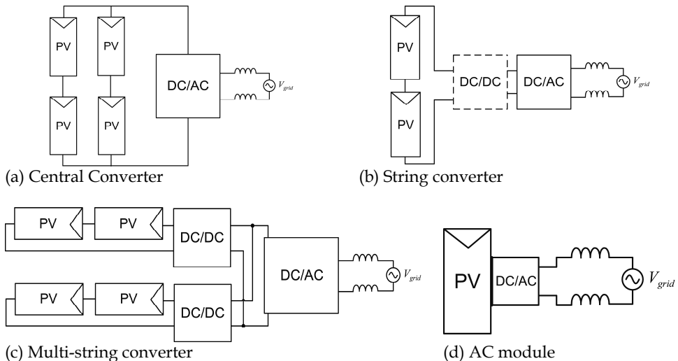
Fig. 4. Configurations of the power converter for a grid connected PV System, central converter (a), string converter (b), multi-string converter (c) and AC module (d).
