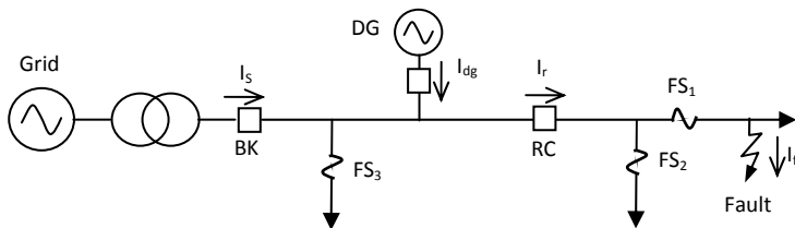
Fig. 1. Change of fault currents due to DG interconnection
