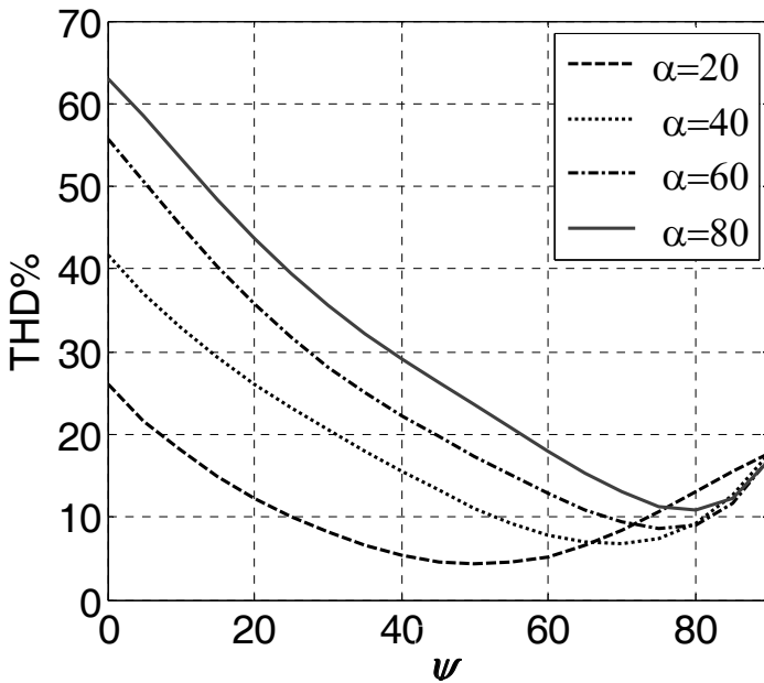
Fig. 8. The relation between THD and the angle of I_f with respect to V_{om} at I_f/I_o=1.15 for different values of firing angle, \alpha .
