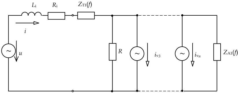
Fig. 3. Equivalent scheme for calculation and state quantities of the network with one R-L appliance for all harmonic components, where Z_{Ti}(f) = i(vf_i) and Z_{Ai}(f) = i(vf_i) = R_1 + j\nu 2\pi f L_{L1} , f_1 is frequency of fundamental harmonic component, i_v are current sources representing nonlinearity of appliance, R = \sum R_v is the sum of source resistances
