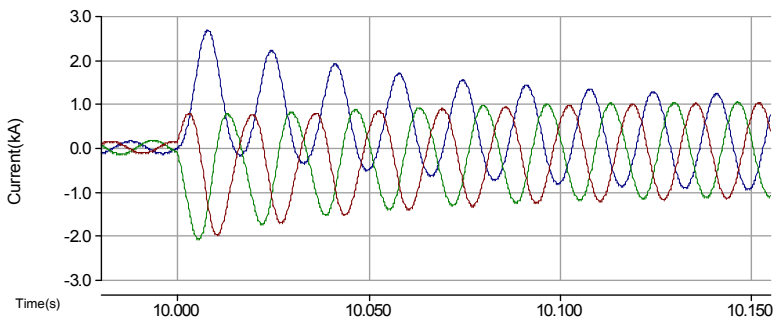
Fig. 10. Fault current contribution from a synchronous generator
