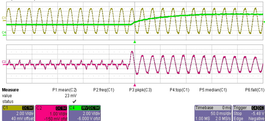
Fig. 18. Steady-state operation of RES in regime of active power delivering: voltage (top) and current (bellow)
