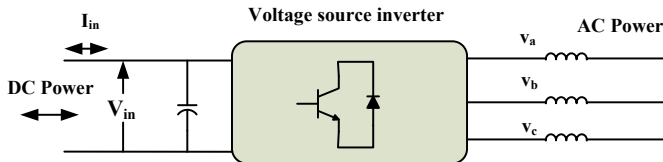
Fig. 5. DC-AC voltage source converter
