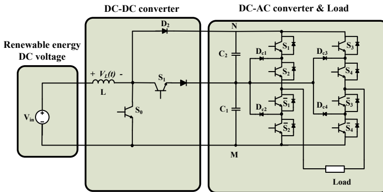
Fig. 17. Three-level diode-clamped topology joint with double-output MOB converter
