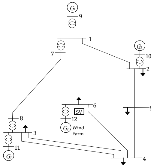
Fig. 23. High voltage transmission system model.
