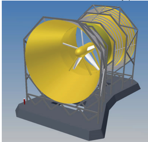
Fig. 17. Tidal turbine with venturi shroud (Source: http://www.reuk.co.uk/Lunar-Energy-Tidal-Power.htm )
