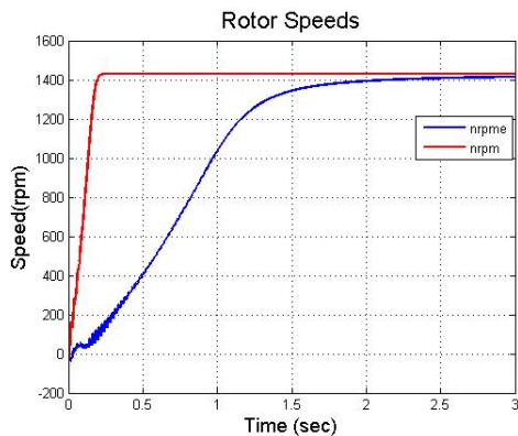
Fig. 12. Estimated rotor speed using EKF
