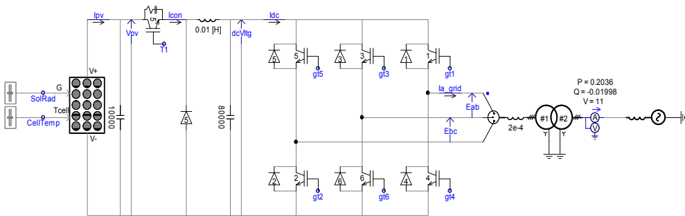
Fig. 14. Schematic of the grid connected PV system simulation (for the simplicity, the ac system is shown as an equivalent source).
