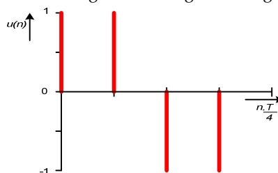
Fig. 12. Switching function for single-phase 2-pulse RES inverter
