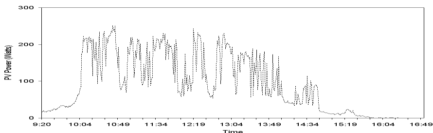
Fig. 18. Photovoltaic power
