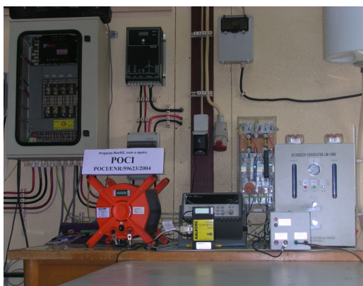
Fig. 4. Stand-alone system's electrolyser, fuel-cell, and electrolyser's DC/DC power converter
