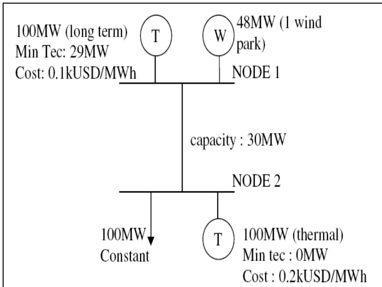
Fig. 7. First study case with simplified transmission system
