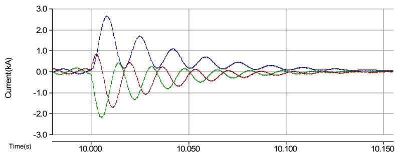
Fig. 12. Fault current contribution from an induction generator with external rotor resistance. Note the faster decay than in the normal induction generator case in Figure 11.
