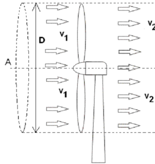
Fig. 4. Flow through a wind energy converter
