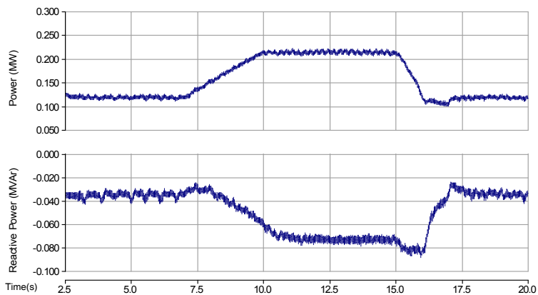
Fig. 17. Real and reactive power output of the inverter
