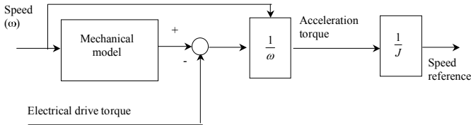
Fig. 10. Calculation of the new speed reference.
