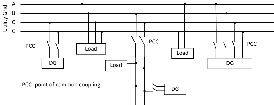
Fig. 3. Possible DG interconnection configurations
