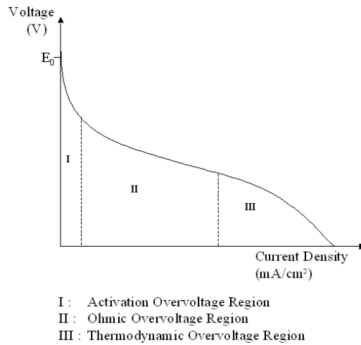
Fig. 8. Fuel cell polarisation curve
