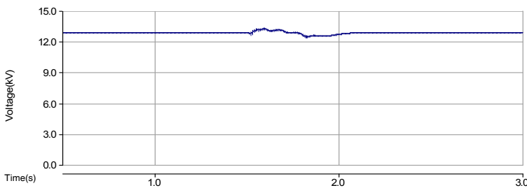
Fig. 8. Voltage at bus 11 during soft starting of the wind generator.
