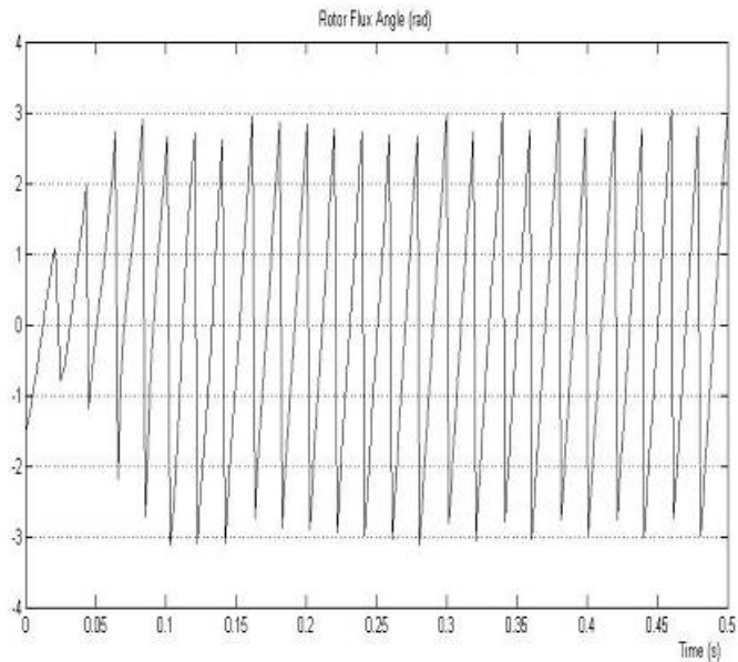
Fig. 19. Estimated rotor flux angle in d-q rotating frame using U_s\text{-}\omega estimator
