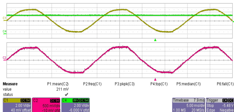
Fig. 20. Steady-state operation of RES in regime of power acceptor from network: voltage (top) and current (bellow)
