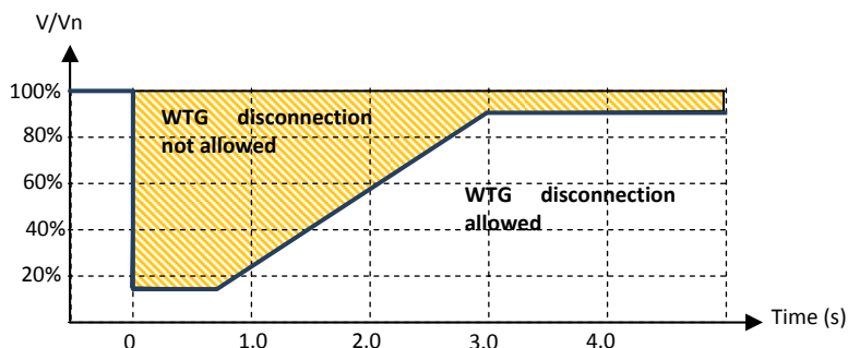
Fig. 21. Typical fault ride through requirements. The actual fault ride through curve can vary depending on the transmission operator.
