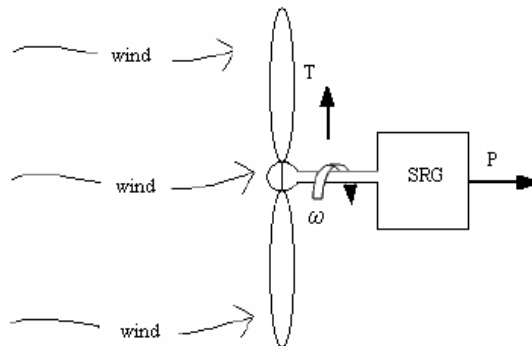
Fig. 11. Direct drive wind turbine with SRG.
