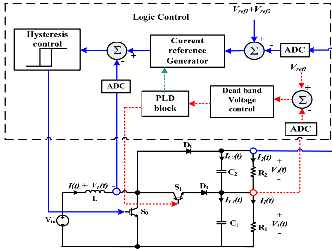
Fig. 19. Block diagram of the proposed control system
