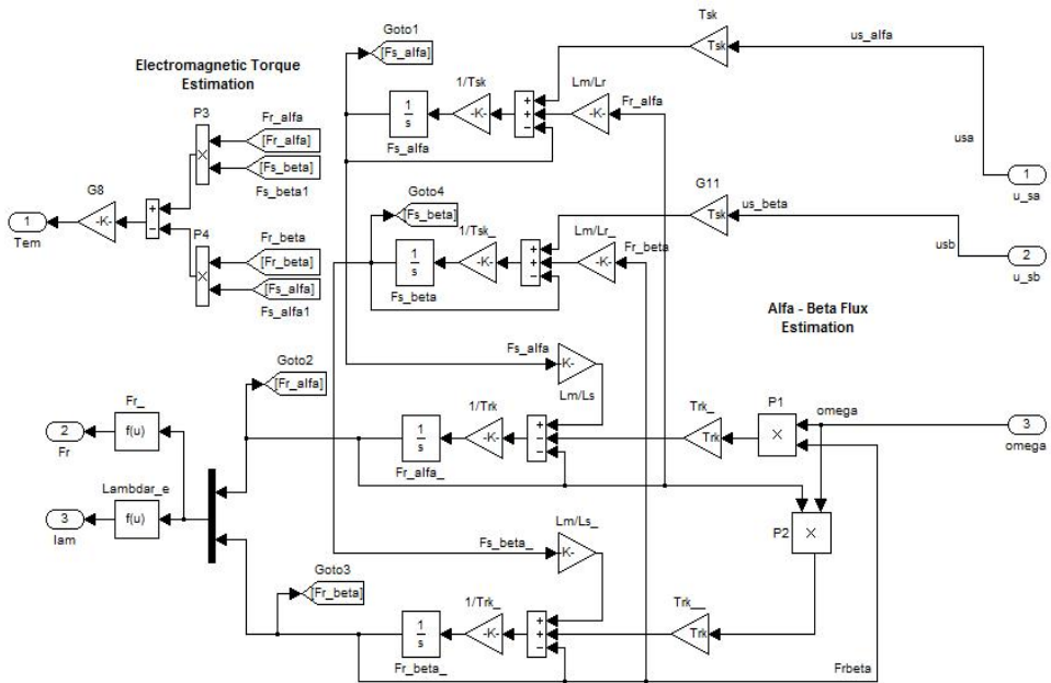
Fig. 17. U_s - \omega estimator Simulink model
