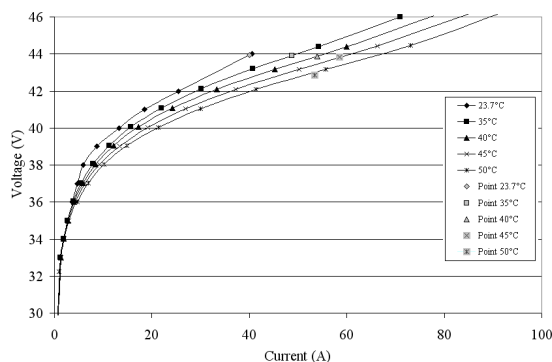
Fig. 7. Stuart electrolyzer polarisation curve
