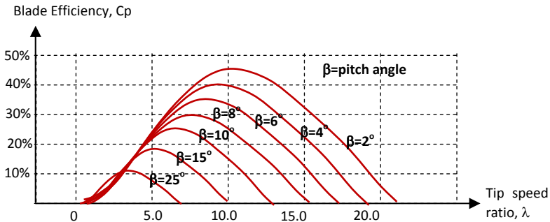
Fig. 22. Typical variation of C_p with wind speed
