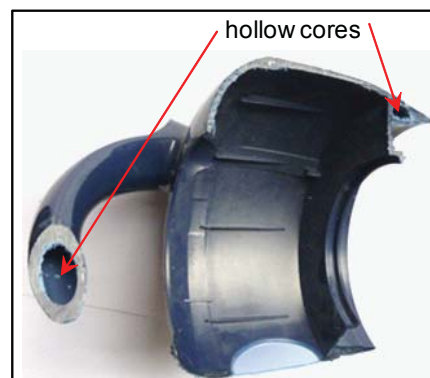
Figure 3.15 A section of a conventional kettle showing the hollow cores
