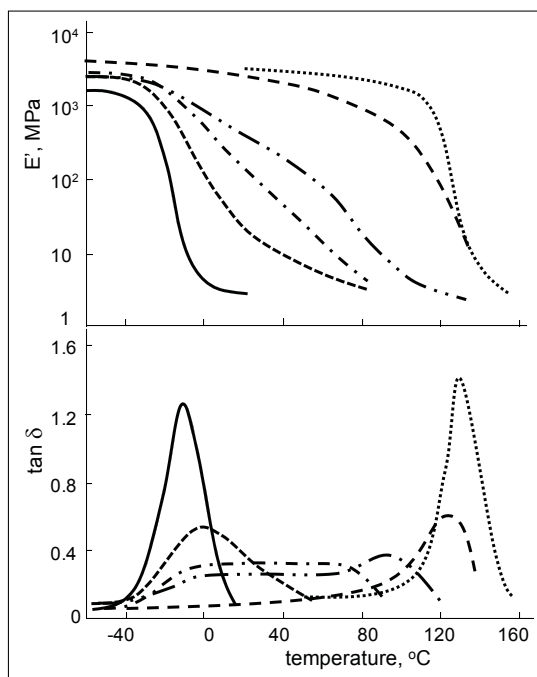
Figure 7.25 E' and \tan \delta vs. temperature for PU/PMMA compositions by weight of (—) 100/0; (---) 80/20; (- . -) 70/30; (- - -) 50/50; (- - -) 20/80 and (.....) 0/100 (source: Akay & Rollins 1993)
