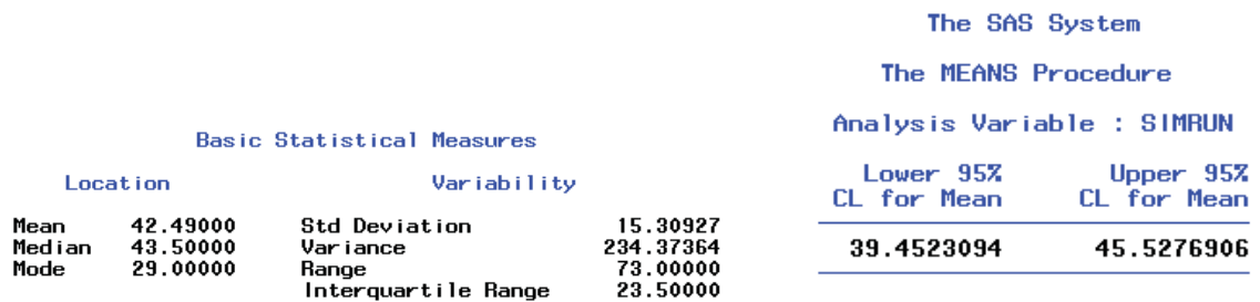
Figure 6.7 Basic Statistical Measures and Confidence Intervals
