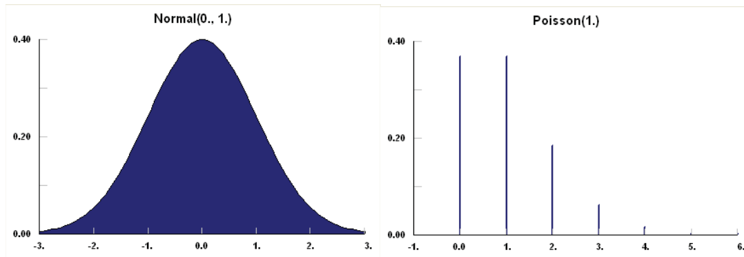
Figure 4.13 Example Distributions
