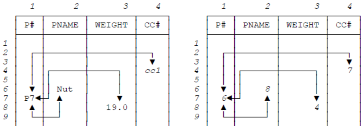
Fig. 14.3: Star for part P7 (with P# the core)
