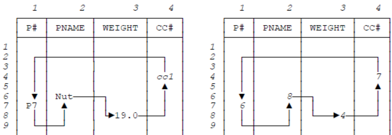
Fig. 14.2: Zigzag for part P7
