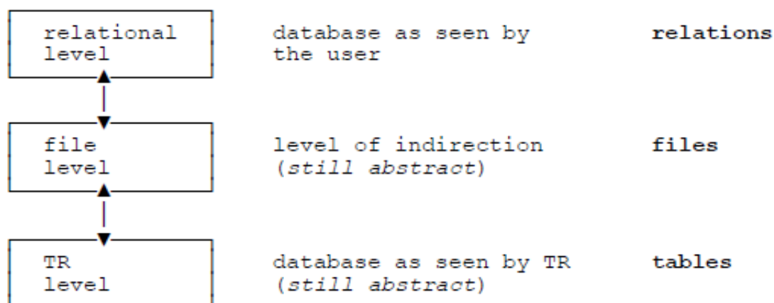
Fig. 3.1: The three levels of abstraction
