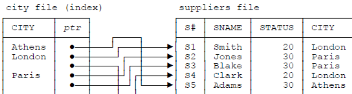
Fig. 2.3: Suppliers with a city index
