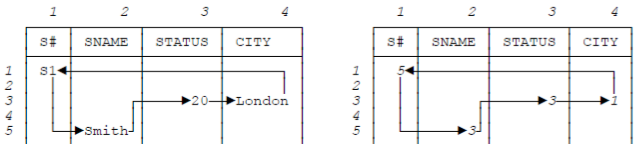
Fig. 4.4: Pointer rings (examples)
